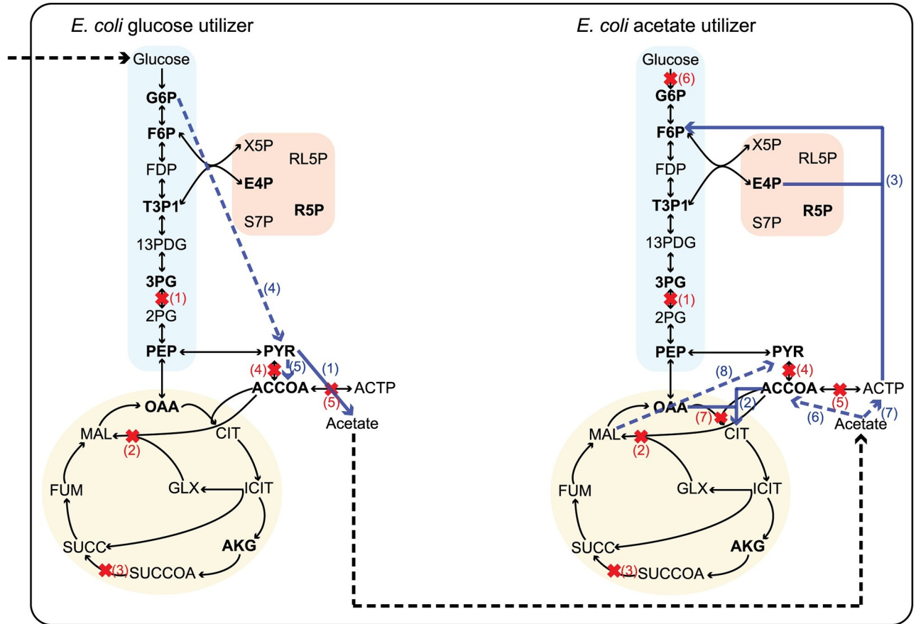
Fig 2. Graphical representation of the toy E. coli community after the application of the community gap-filling method. The central carbon metabolism of an E. coli core model (blue rectangular: Glycolysis, pink square: Pentose Phosphate Pathway, yellow circle: TCA cycle) was used in order to create two E. coli strains: one that consumes glucose (left) and one that consumes acetate (right), after the deletion of the reactions marked with red crosses. The best solution of the community gap-filling algorithm predicted the addition of the reactions represented by continuous blue arrows and the activation of the existing reactions represented by dashed blue arrows, in order to restore biomass production in the two models. The dashed black arrows show the exchange reactions for glucose and acetate in the community. The metabolites in bold represent biomass precursors. The numbered deleted reactions are: (1) PGM, (2) MALS, (3) SUCOAS, (4) PFL, (5) PTAr, (6) GLCpts, (7) CS. The numbered added and activated reactions are: (1) POX, (2) CS, (3) PKETF, (4) EDD and EDA, (5) PDH, (6) ACS, (7) ACKr, (8) ME1.
