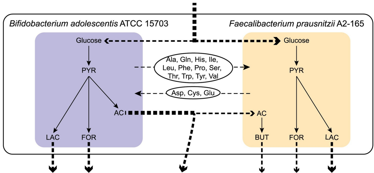
Fig 3. Graphical representation of the community of B. adolescentis ATCC 15703 and F. prausnitzii A2-165 after the application of the community gap-filling method. The best solution calculated by the community gap-filling algorithm predicted that the metabolic models of the strains B. adolescentis ATCC 15703 and F. prausnitzii A2-165 share the available Glucose from the common medium and produce lactate (LAC), formate (FOR), and butyrate (BUT), while they exchange acetate (AC), and amino acids (3 letter code). The non-dashed arrows represent intracellular metabolite flow and the dashed arrows represent the exchange reactions of SCFAs and amino acids. The thickness of the dashed arrows represents the relative order of magnitude of the calculated fluxes for the exchange reactions.
