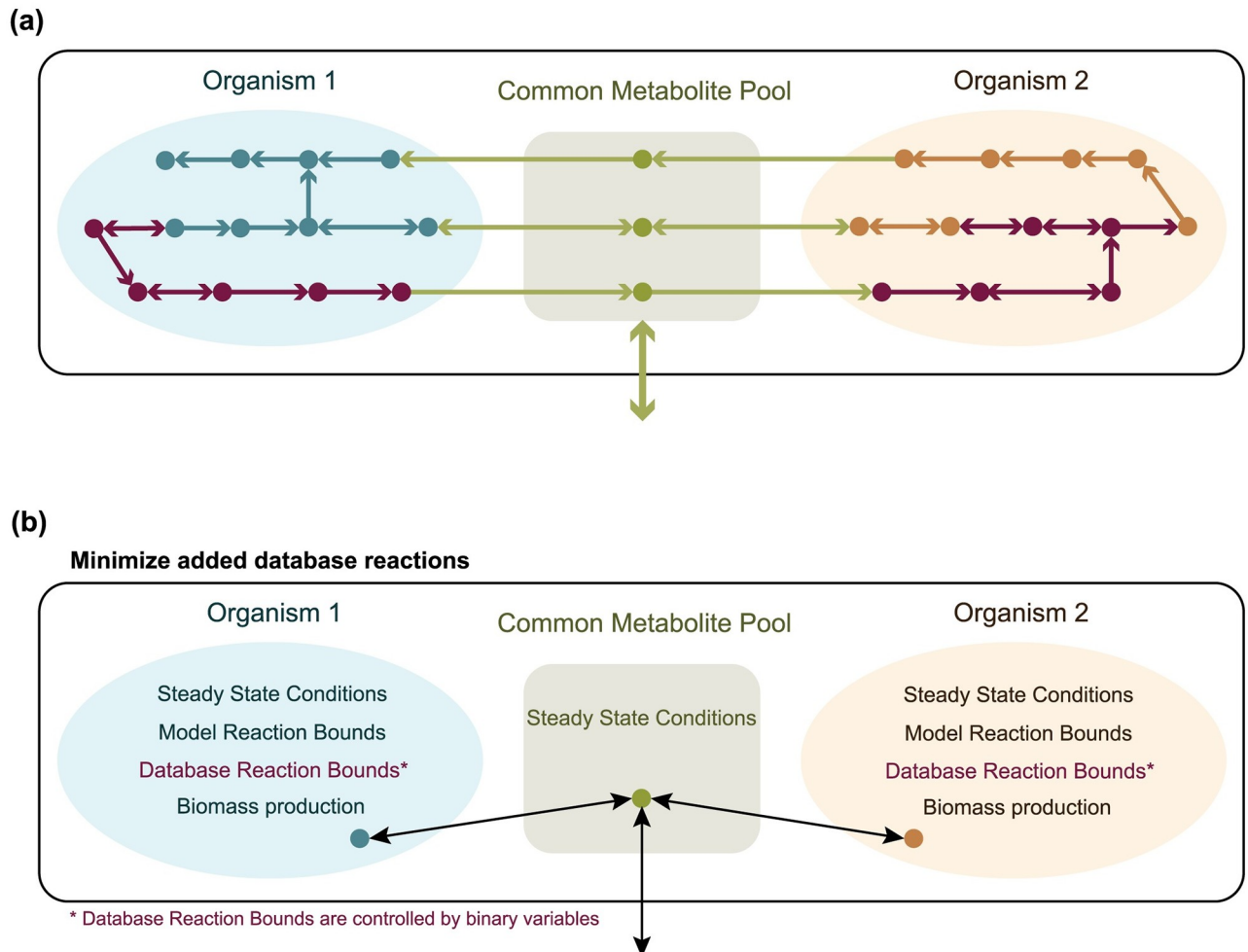
Fig 1. Graphical representation of the community gap-filling method. The metabolic reconstructions of two individual organisms (blue and orange respectively) are allowed to exchange metabolites and interact with the environment through a common metabolite pool (green). (a) The algorithm adds biochemical reactions from a reference database (dark purple) to the community model. (b) The community gap-filling algorithm is an MILP problem with the objective to add the minimum number of database reactions to the community model in order to restore biomass production in the individual metabolic models, while it satisfies some constrains for the reaction fluxes. In each compartment of the community model, the metabolite pools are assumed to be in steady state. The addition of each database reaction is controlled by a binary variable, which takes the value of 1 if the database reaction is added to the community model, and 0 otherwise.
