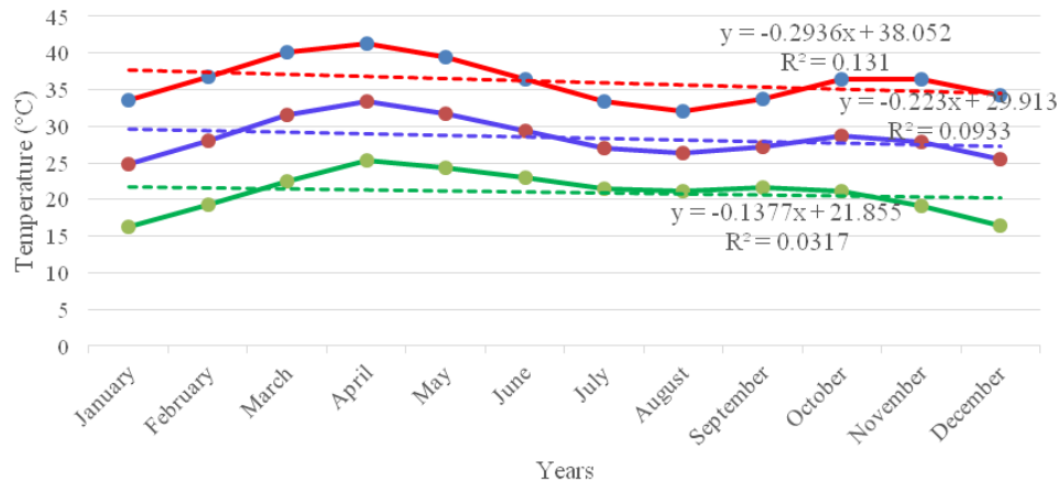
Fig. 13. Monthly variation in maximum, mean and minimum temperatures (in red, blue and green, respectively) at the Maroua weather station
