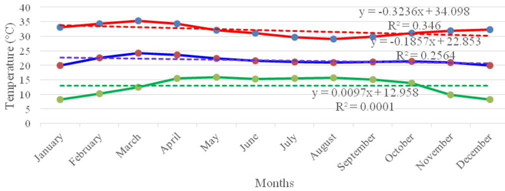
Fig. 5. Monthly variation in maximum, mean and minimum temperatures (in red, blue and green, respectively) at the Ngaoundere weather station
