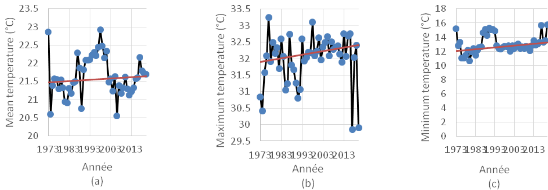
Fig. 4. Mann-Kendall tests were applied to analyze the trend of mean temperature (a), maximum temperature (b) and minimum temperature (c) in Ngaoundere
