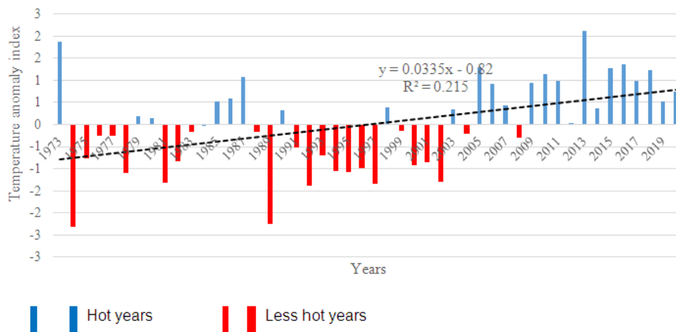
Fig. 7. Mean temperature anomaly index in Garoua
