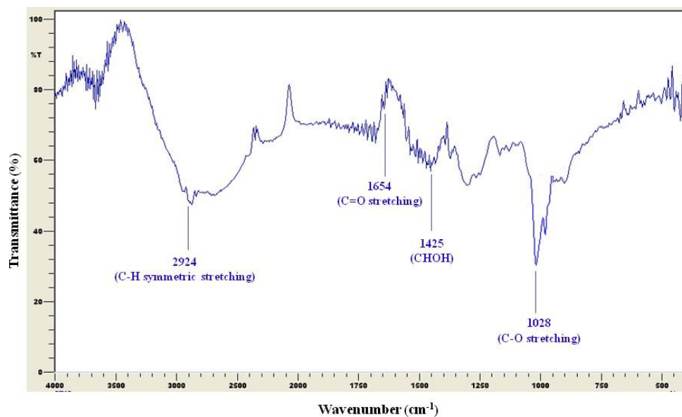
Fig. 6. FTIR spectra of Chitosan
