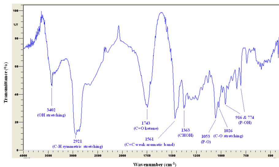
Fig. 8. FTIR spectra of rutin, chitosan and sodium TPP
