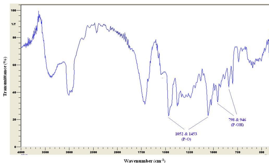
Fig. 7. FTIR spectra of Sodium TPP
