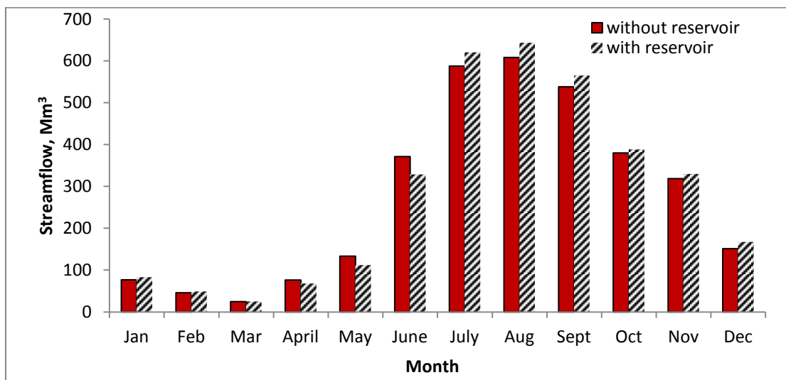
Fig. 8. Monthly streamflow with and without reservoirs (0.1% increase in area of waterbodies) during 2041-2070 under RCP8.5
