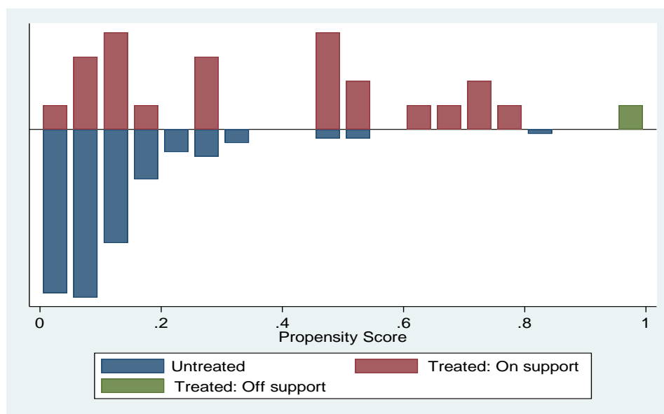
Fig. 1. Propensity scores distribution
