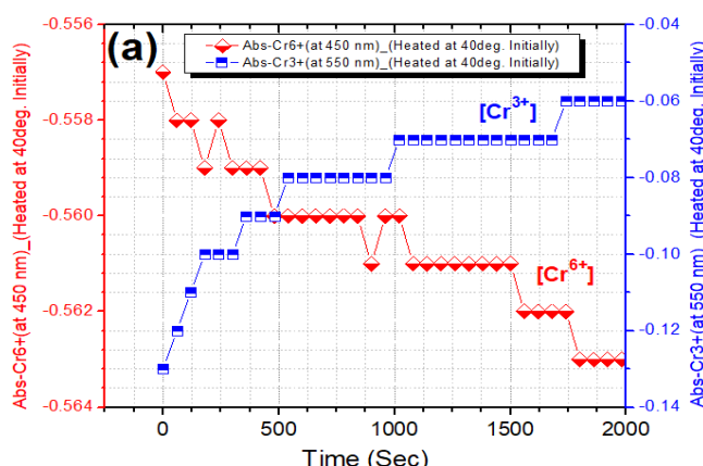
Fig. 9(a). Kinetic profile that represents the conversion of Cr(VI) reactant to Cr(III) product under heated conditions
