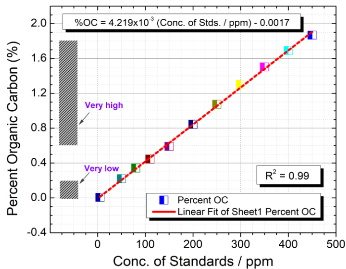
Fig. 11. Conversion chart for the estimation of %OC in soil samples
