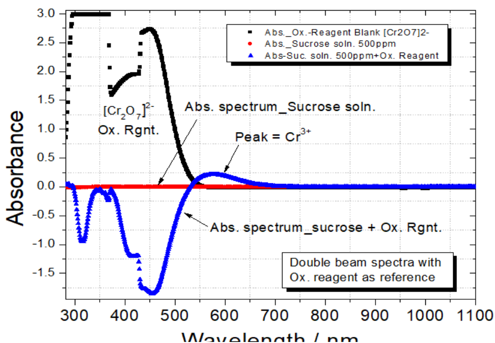
Fig. 1. Electronic Absorption Spectrum of Oxidizing Reagent (reference blank), Sucrose Solution (reference blank) and Sucrose Solution (Treated with the Oxidizing Agent)
