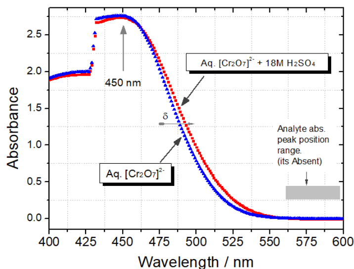
Fig. 6. Broadening of the dichromate ion absorption band due to addition of 18M H 2 SO 4 acid
