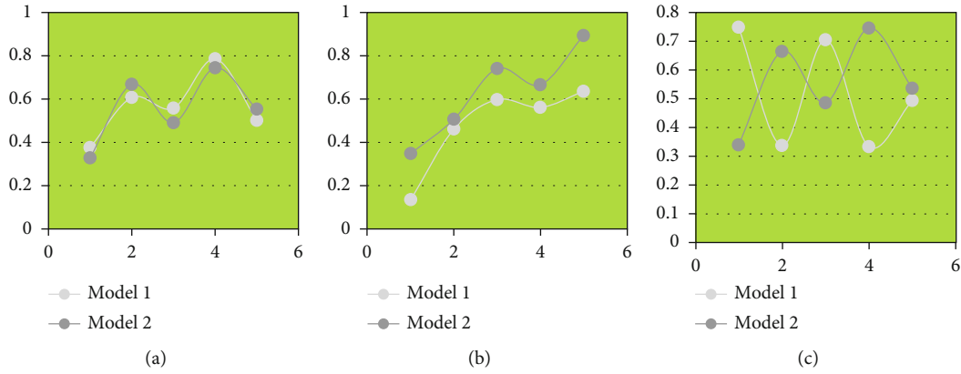
FIGURE 6: Similarity measurement.
