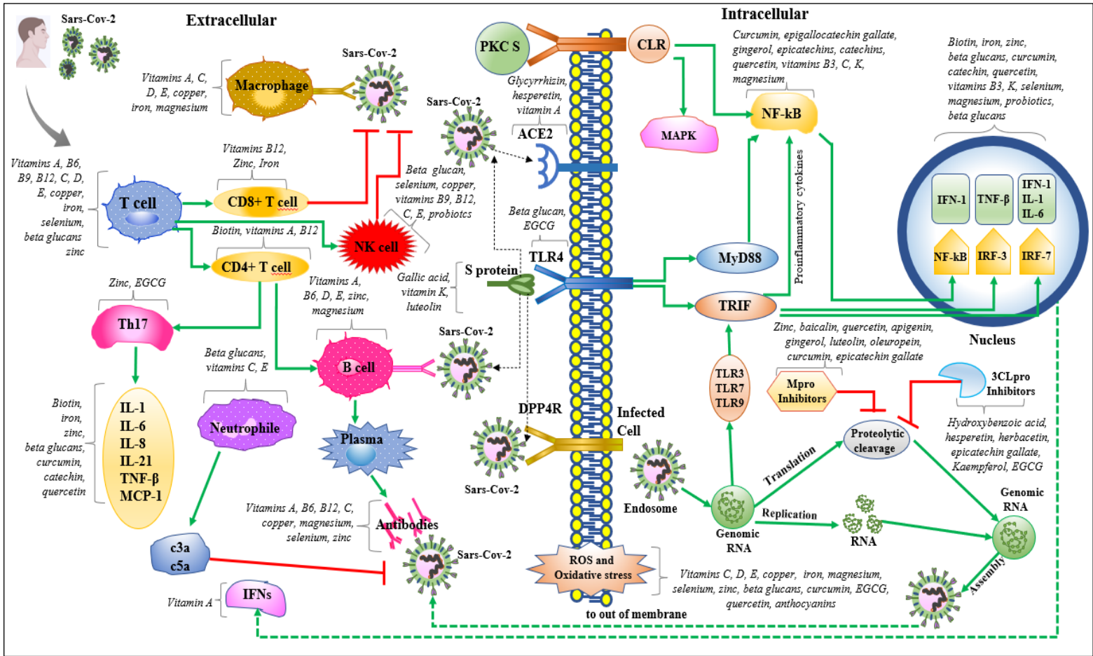
Fig. 1. Immune responses against SARS-CoV-2 and contributions of some micronutrients and bioactive compounds to various cell and cytokines involved in the defense mechanism during infection (red lines refer to inhibitory effects; green lines refer to activating effects). Adapted from Li et al. [24] and Arruda de Souza Monnerat et al. [246]
